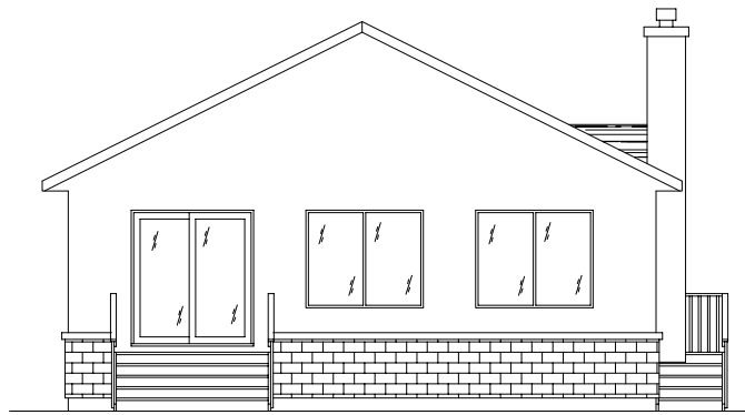
FRONT ELEVATION
